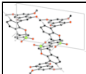
Fig. 2. The packing of (I), viewed down the b axis. Hydrogen bonds are shown as dashed lines. H atoms not involved in hydrogen bonding have been omitted.
